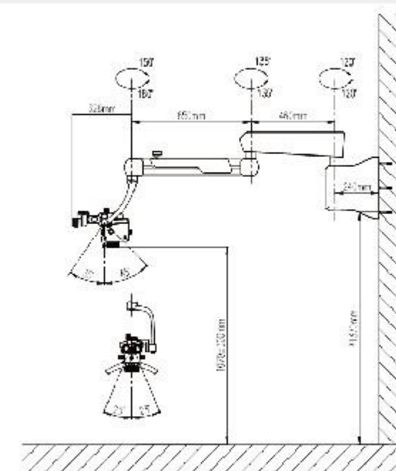
Low position wall mount
