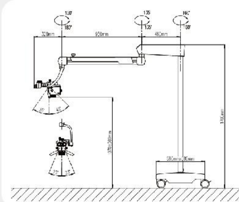
Floor stand with 950 pantograph arm
