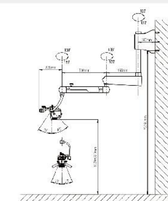
High position wall mount
