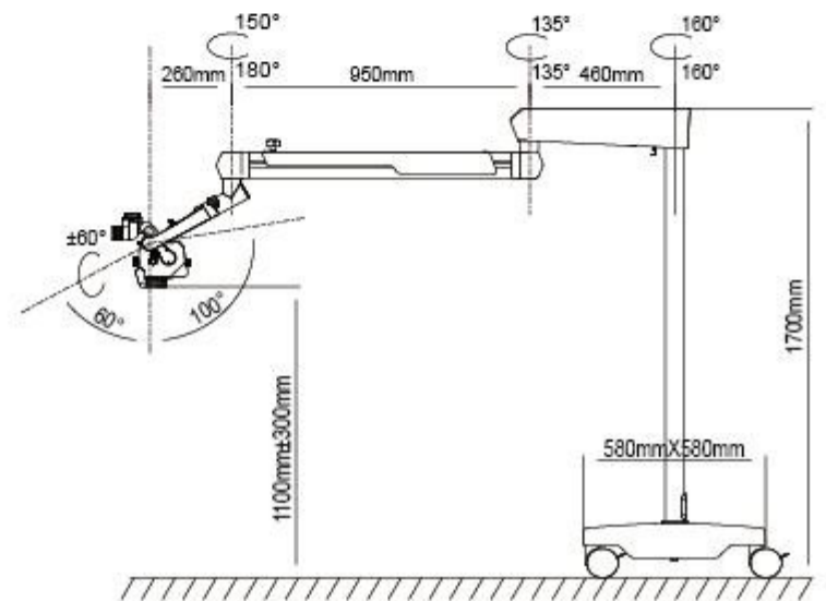
Floor stand with 950 pantograph arm
