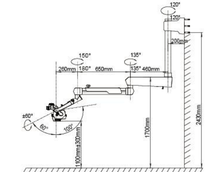
High position wall mount
