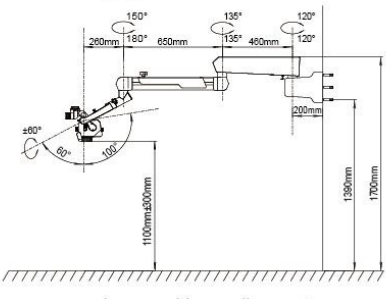
Low position wall mount
